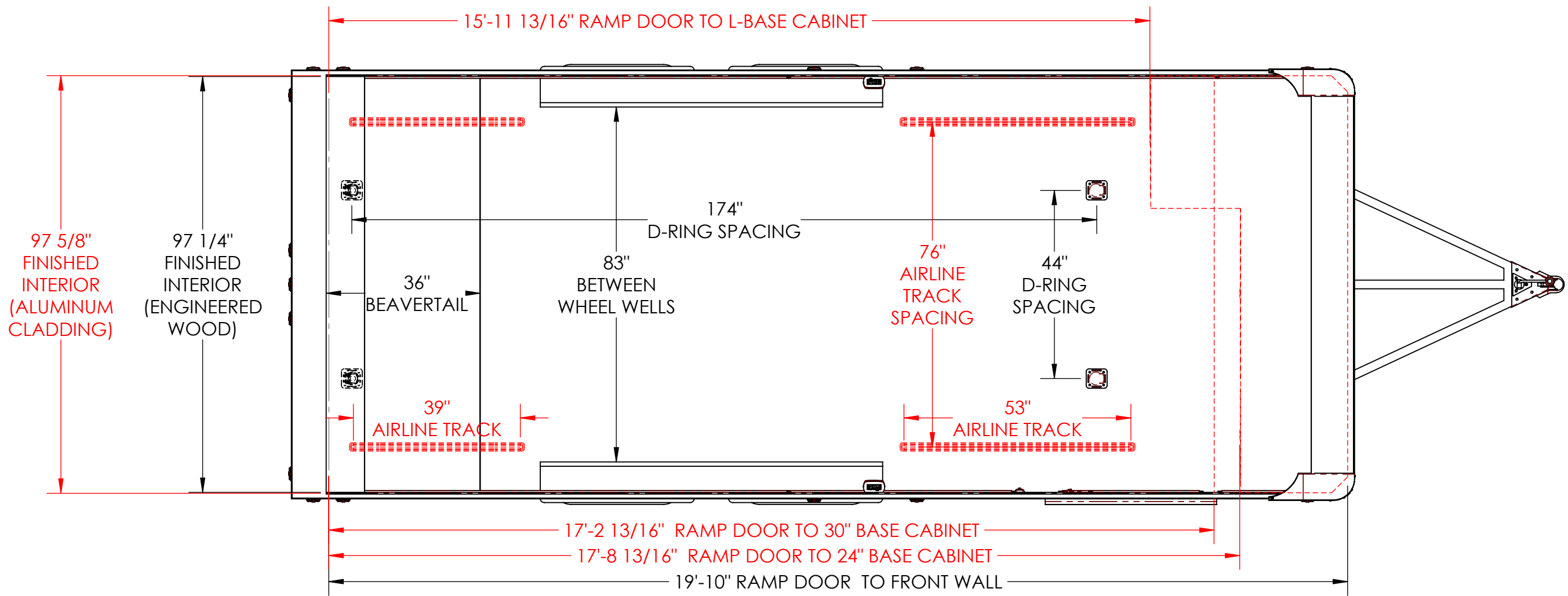
TOP VIEW FLOORPLAN LAYOUT
