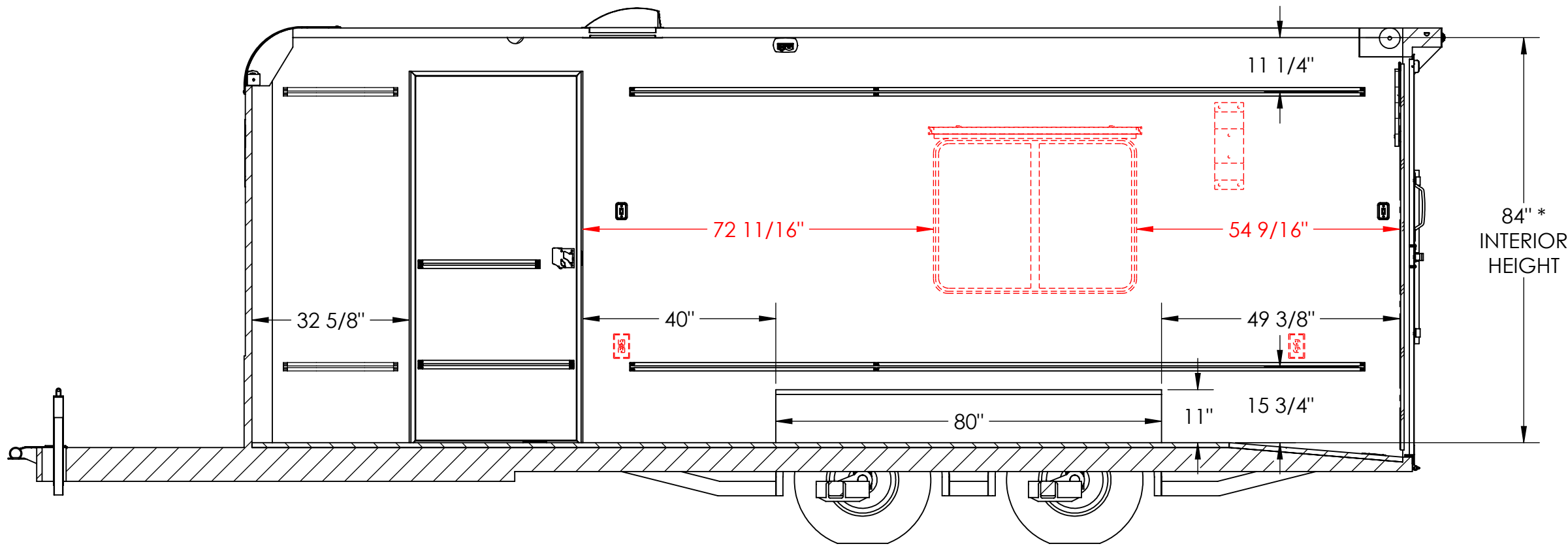
INTERIOR CURB SIDE SECTION B-B
