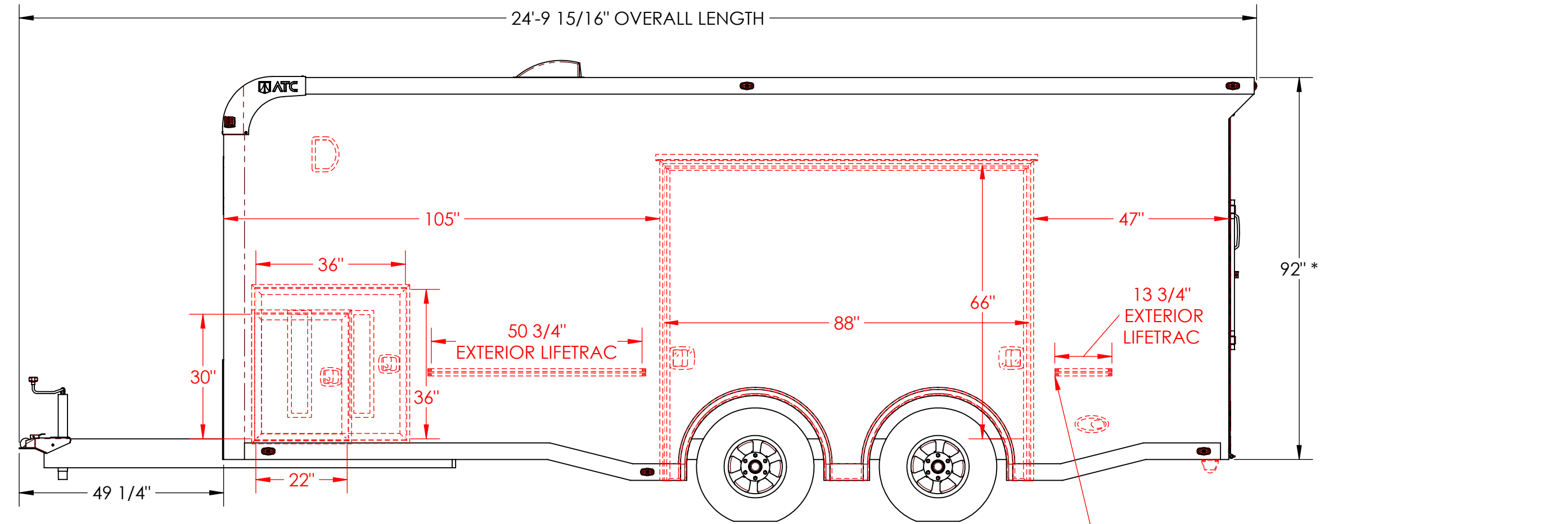
EXTERIOR CURB SIDE
