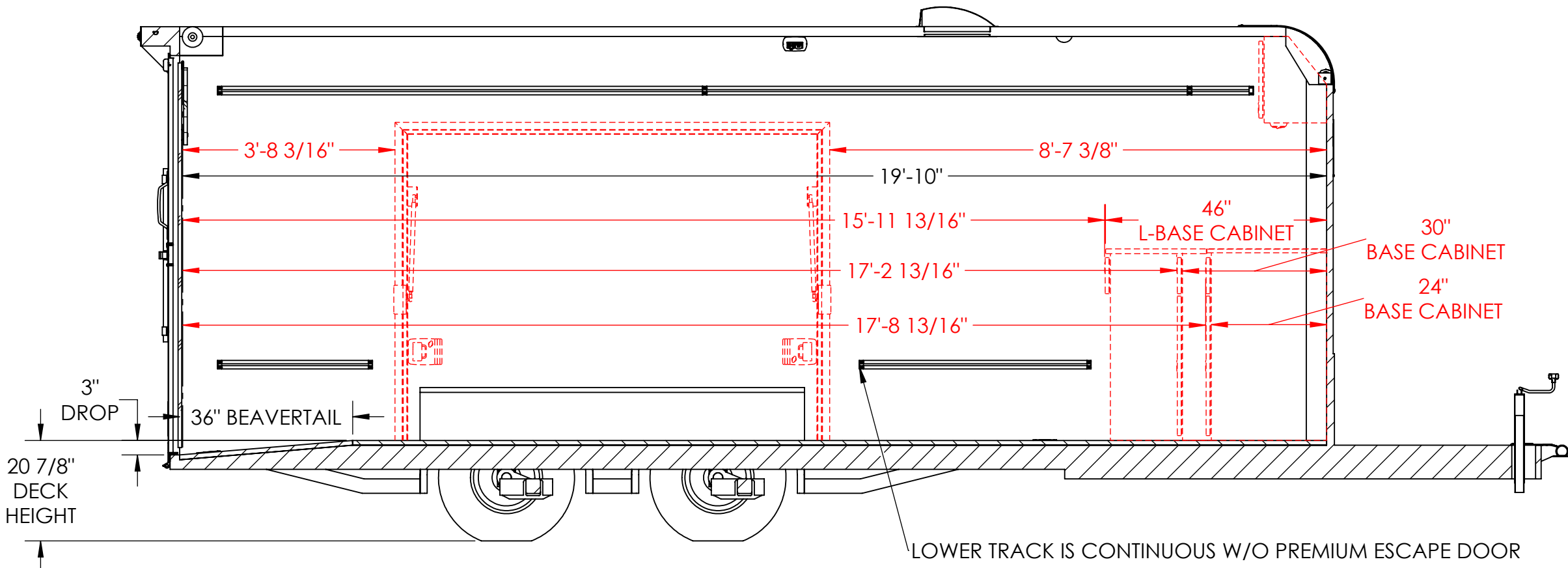
INTERIOR ROAD SIDE SECTION A-A
