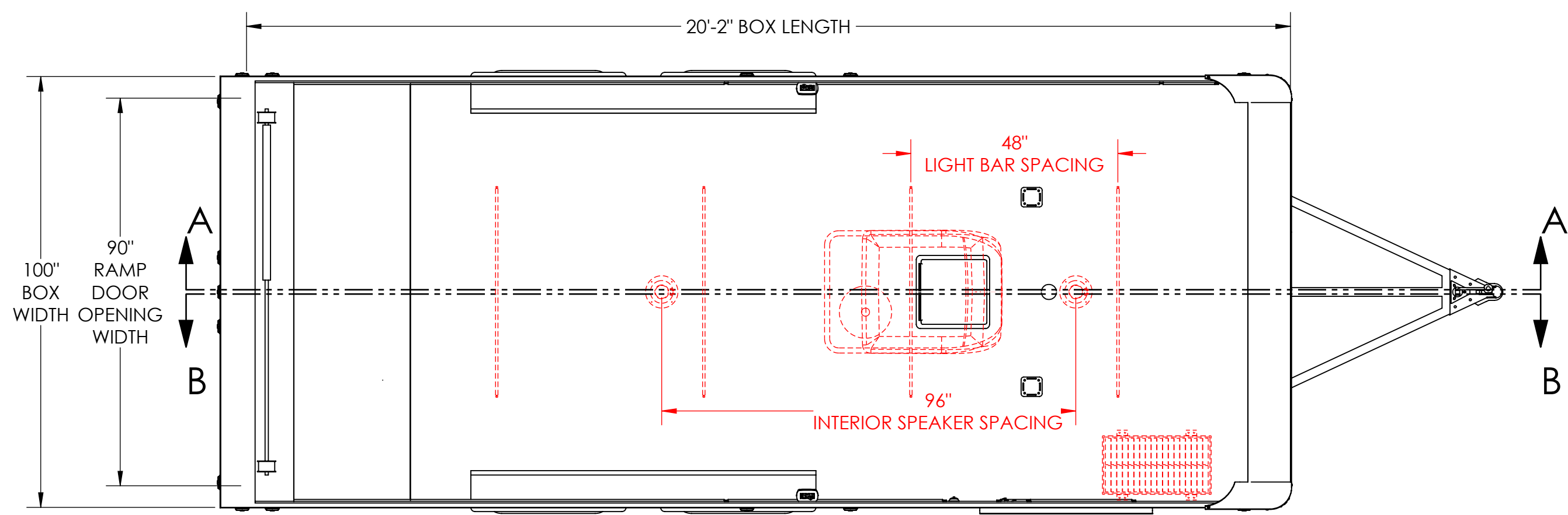
TOP VIEW ROOF & CEILING LAYOUT
